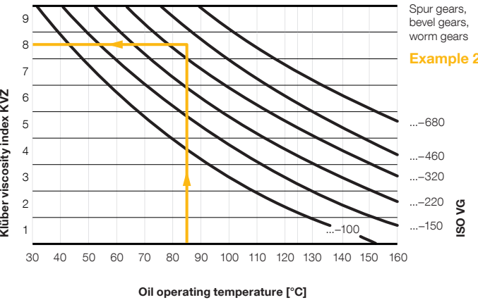
Viscosity selection for Klübersynth UH1 6
