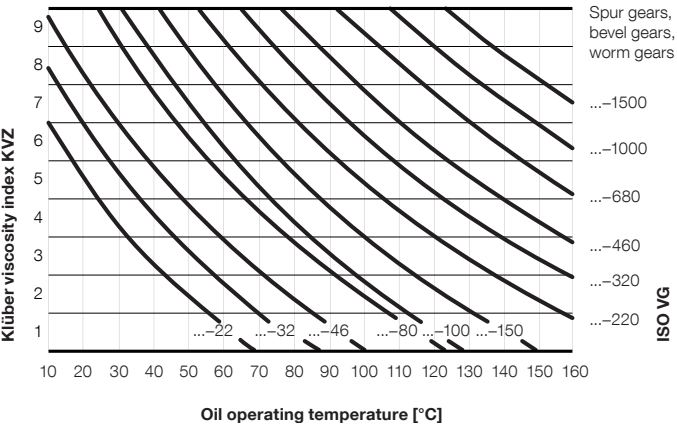
Viscosity selection for Klübersynth GH 6
