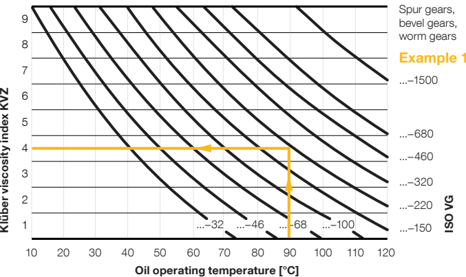
Viscosity selection for Klüberoil 4 UH1 N
