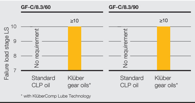
FZG micropitting test (results)
