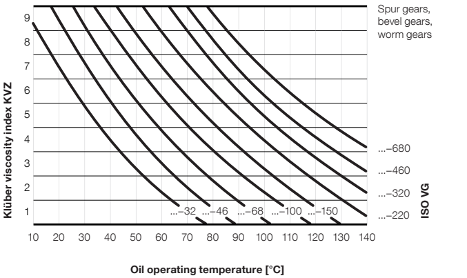
Viscosity selection (ISO VG) for Klübersynth GEM 4 N
