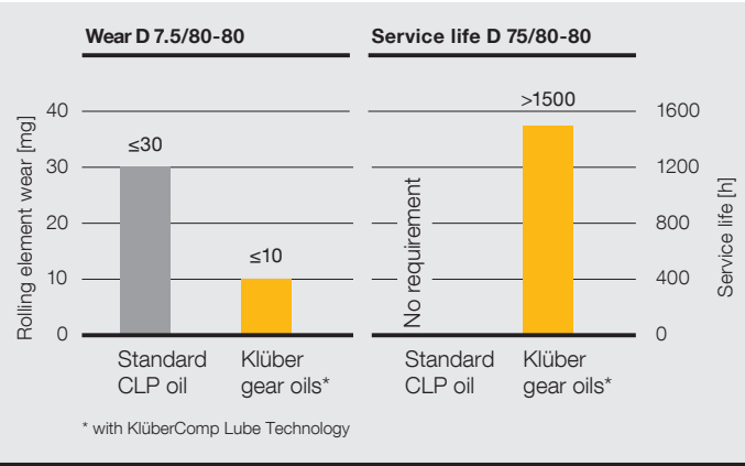
FE8 rolling bearing test (results)
