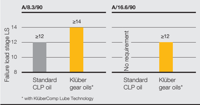
FZG scuffing test (results)
