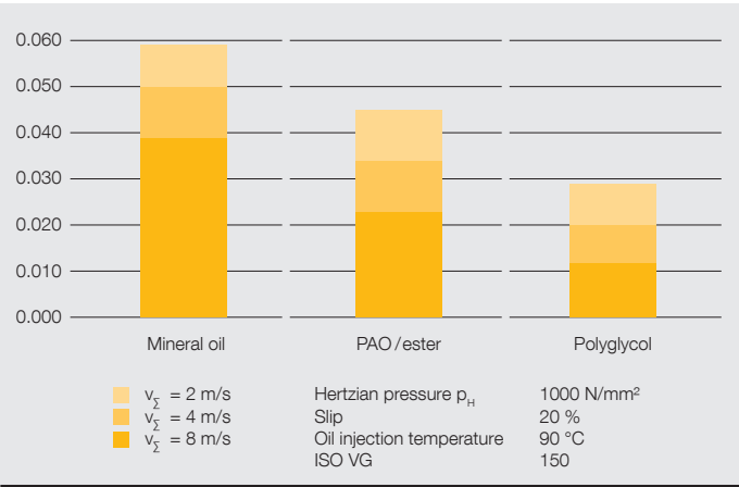
Friction coefficients of various gear oils determined on the twin-disk machine
