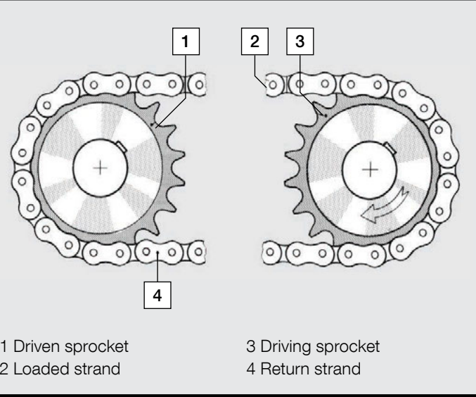
Schematic view of a chain drive
